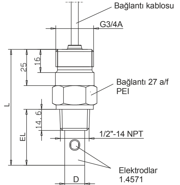
Tip 202922/20-0010-1003-60-144-20-5000-040 Hücre sabiti K = 0.1 Tip 202922/20-0001-1003-26-144-20-5000-063 Hücre sabiti K = 0.01
