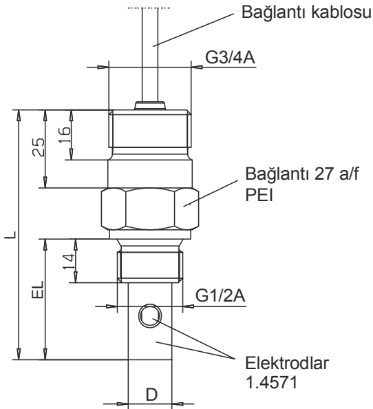
Tip 202922/20-0010-1003-26-104-20-5000-040 Hücre sabiti K = 0.1 Tip 202922/20-0001-1003-26-104-20-5000-063 Hücre sabiti K = 0.01
