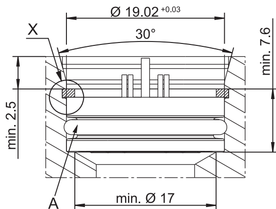
(A) O-ring 16×1.8
