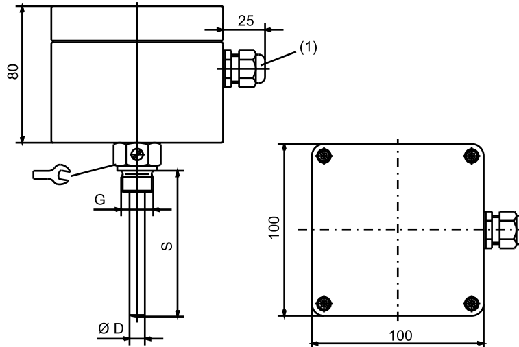
ATHs-SW (Type 603035/...-1-...) with process connection screw-in thermowell
