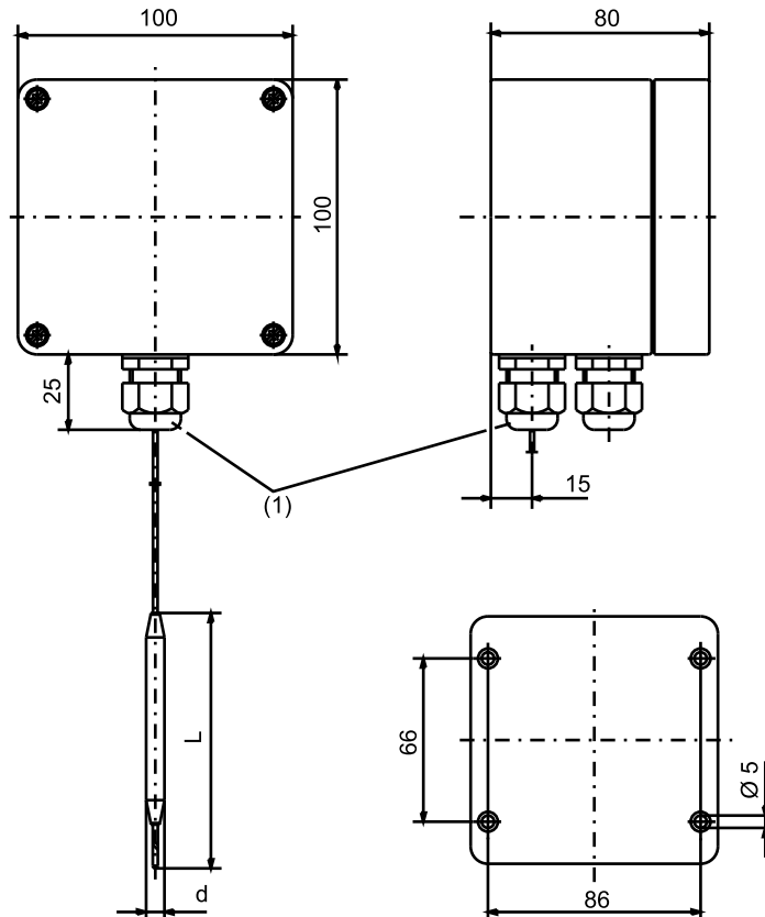
ATHf-SW (Type 603035/...-2-...) with capillary and process connection plain cylindrical probe
